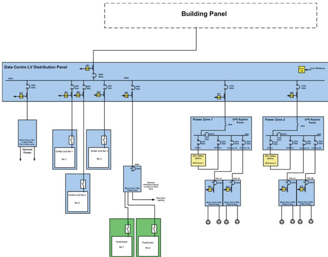
Example EcoMeasure Electrical Drawing
